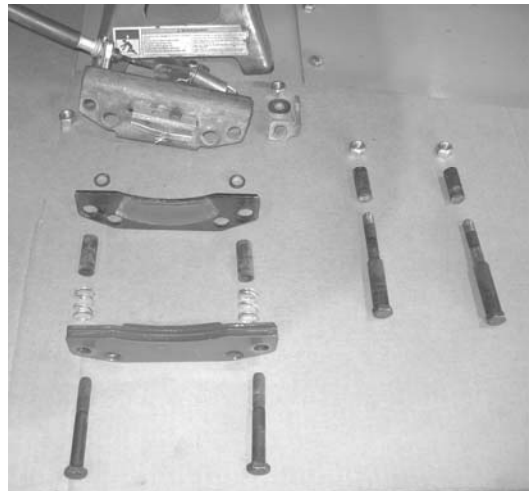
Fig R4 - disassembly
