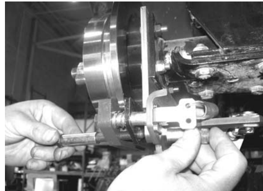
Fig. R9 - Back view of caliper.
