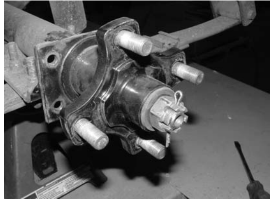
Fig. 4 Install splined hub
